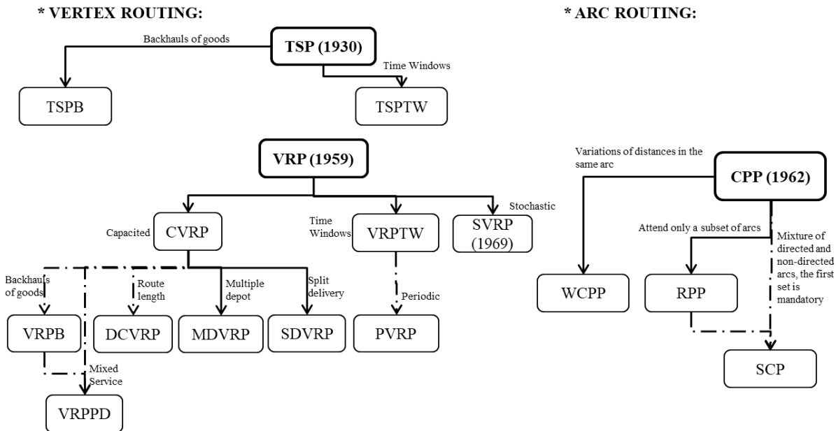
Figure 1. Classification of vehicle routing models [19].
