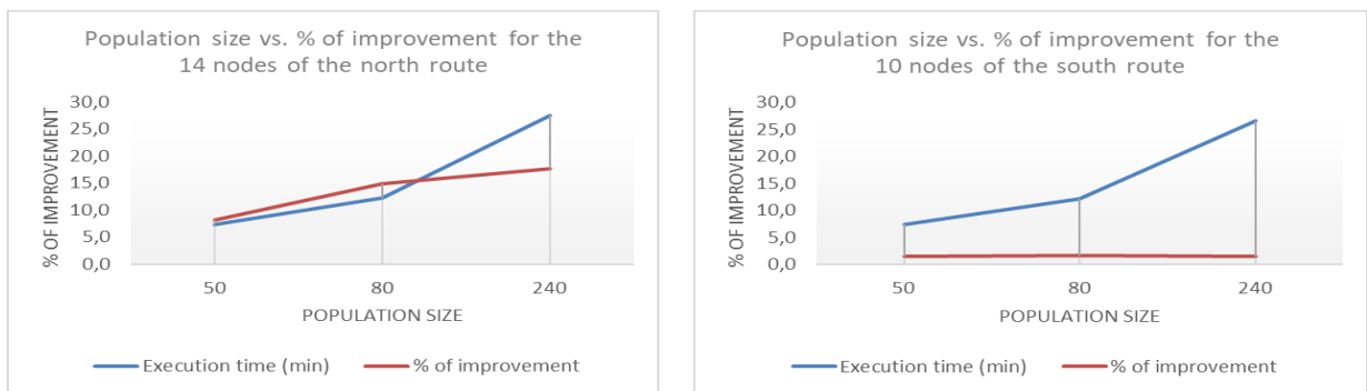
Figure 10– Changing the population size at the GA
