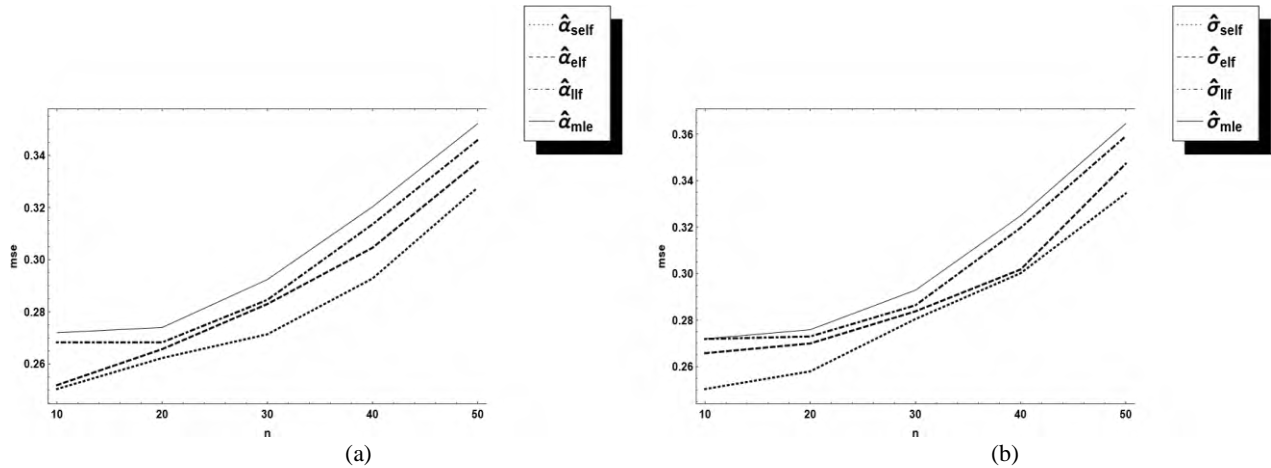
Figure 1: MLE and Bayes estimators of the \alpha and \sigma under different loss functions based on the M-H Algorithm
